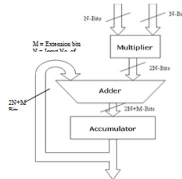
Fig.4 Architecture of MAC Unit
