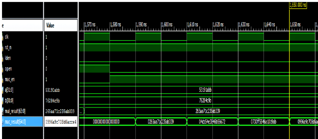
Fig 7. Simulation w/f of proposed 32-bit MAC Unit
