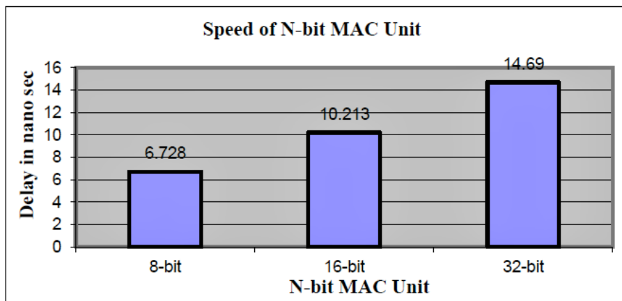
Fig 8. Speed of N-bit MAC Unit
