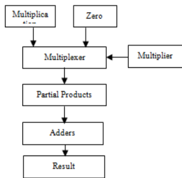
Fig.3 Architecture of conventional multiplier.
