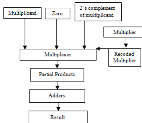
Fig 2. Architecture of Booth Multiplier
