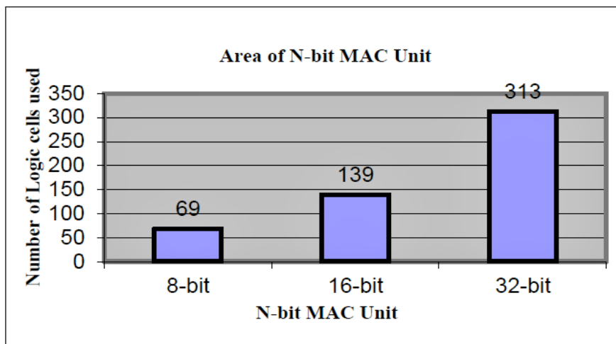
Fig 9. Area of N-bit MAC Unit
