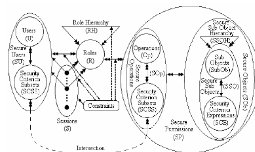
CB-RBAC MODEL
