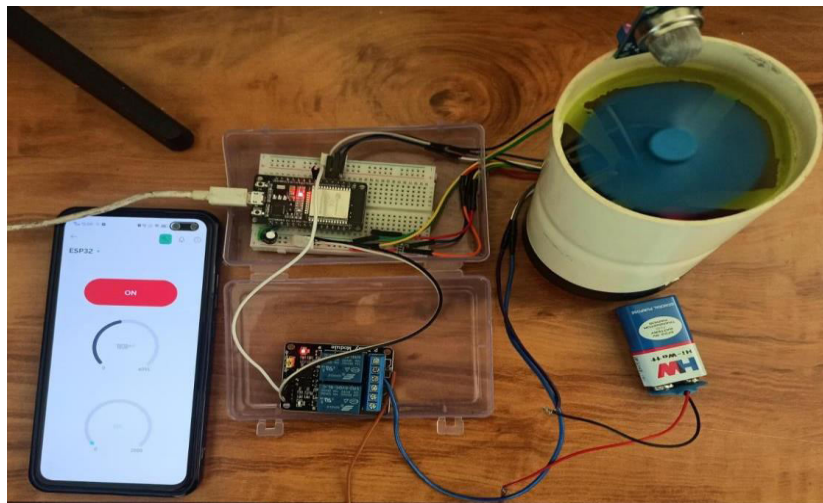
Figure .2 Dust collection System
