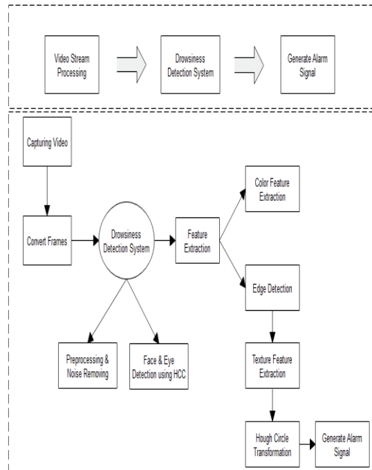
Fig.2 System Architecture
