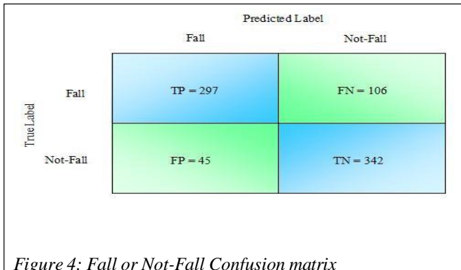
Figure 4: Fall or Not-Fall Confusion matrix
