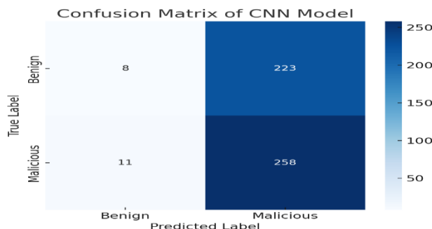
fig. 3. The Cnn Model's Accuracy In Classifying Benign And Malicious Traffic. It Provides Insights Into Prediction Performance
