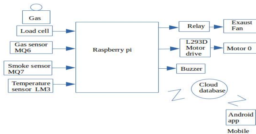
Fig1:- LPG Level Monitoring, Booking & Gas Leakage Detector
