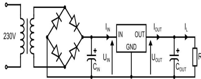
Fig.12 Power supply circuit
