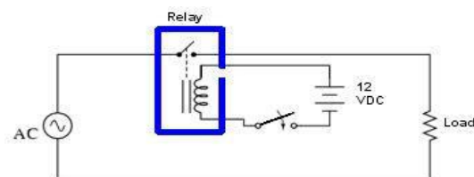
Fig.11 Relay circuit
