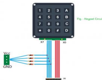
Fig.7 Keypad
