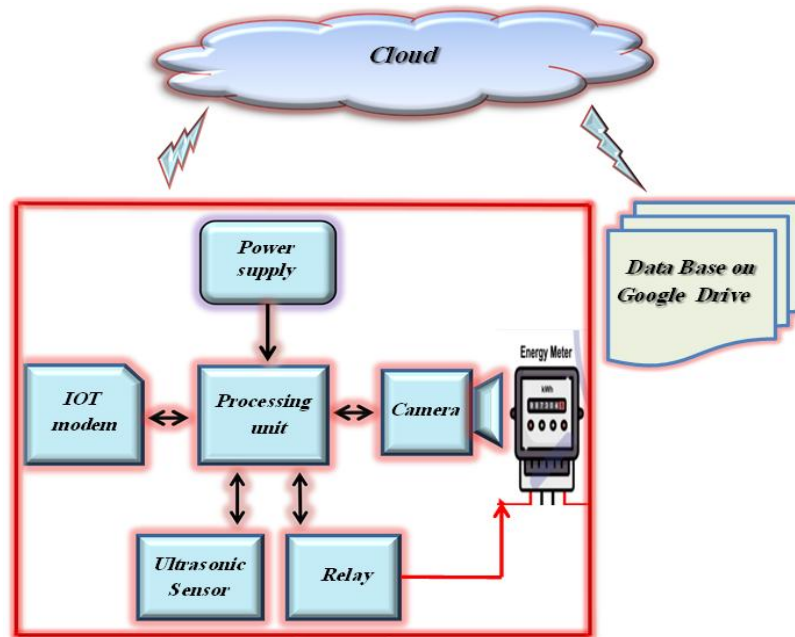
Fig.1 . The Block Diagram of the Proposed Electrical Energy Meter System
