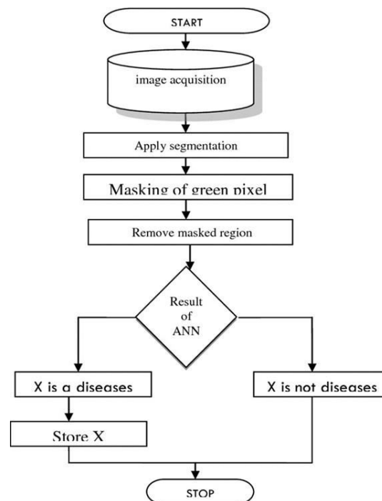
Fig 2: Flowchart for leaf classification
