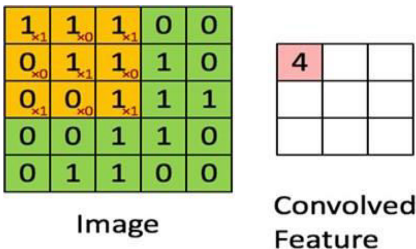
Fig 5: convoluting a 5x5x1 image with a 3x3x1 kernel to get a 3x3x1 convolved feature
