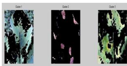
Fig 4: Image clustering
