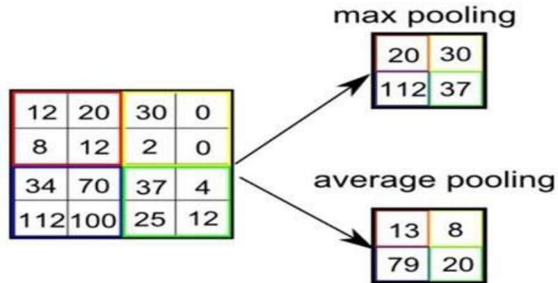
Fig 6: selecting maximum and average pooling matrix
