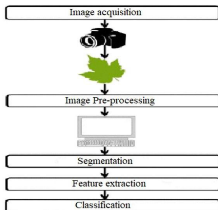
Fig 3: System Architecture
