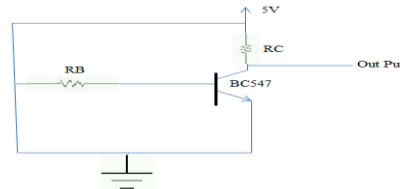
Figure 7: Transistor as a switch
