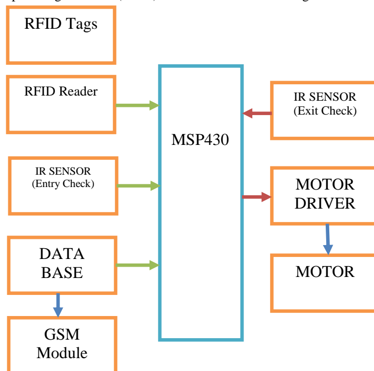
Fig2: Block diagram of automated toll-ticketing
