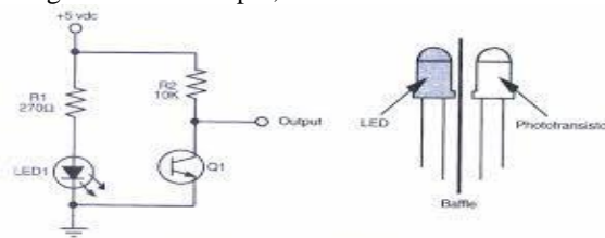
Figure 3 : IR Proximity Sensor
