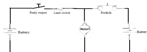
Figure 6: Gate Operation Circuit
